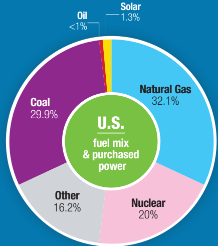
Major energy sources and percent share of total U.S. electricity generation in 2018.
