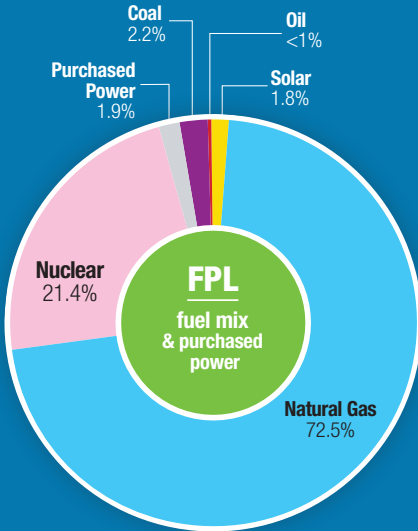
Sources of electricity generation for the 12 months that ended September 2019.
